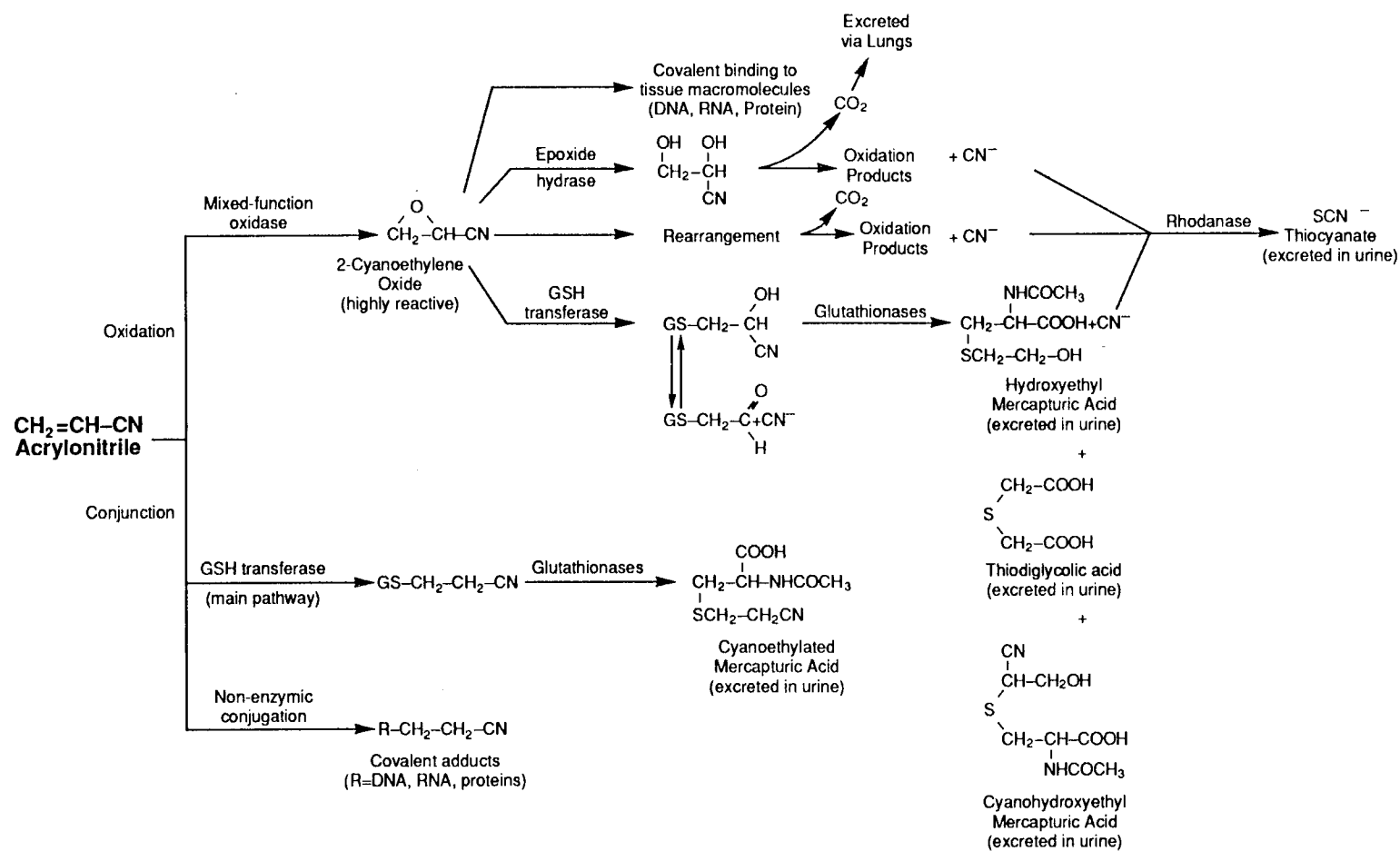
FIGURE 2-3. Proposed Metabolic Scheme for Acrylonitrile
